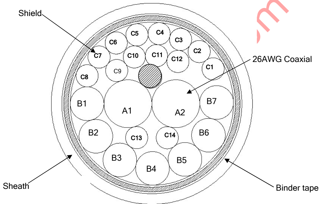
Fig.2 Cross section view of cable
