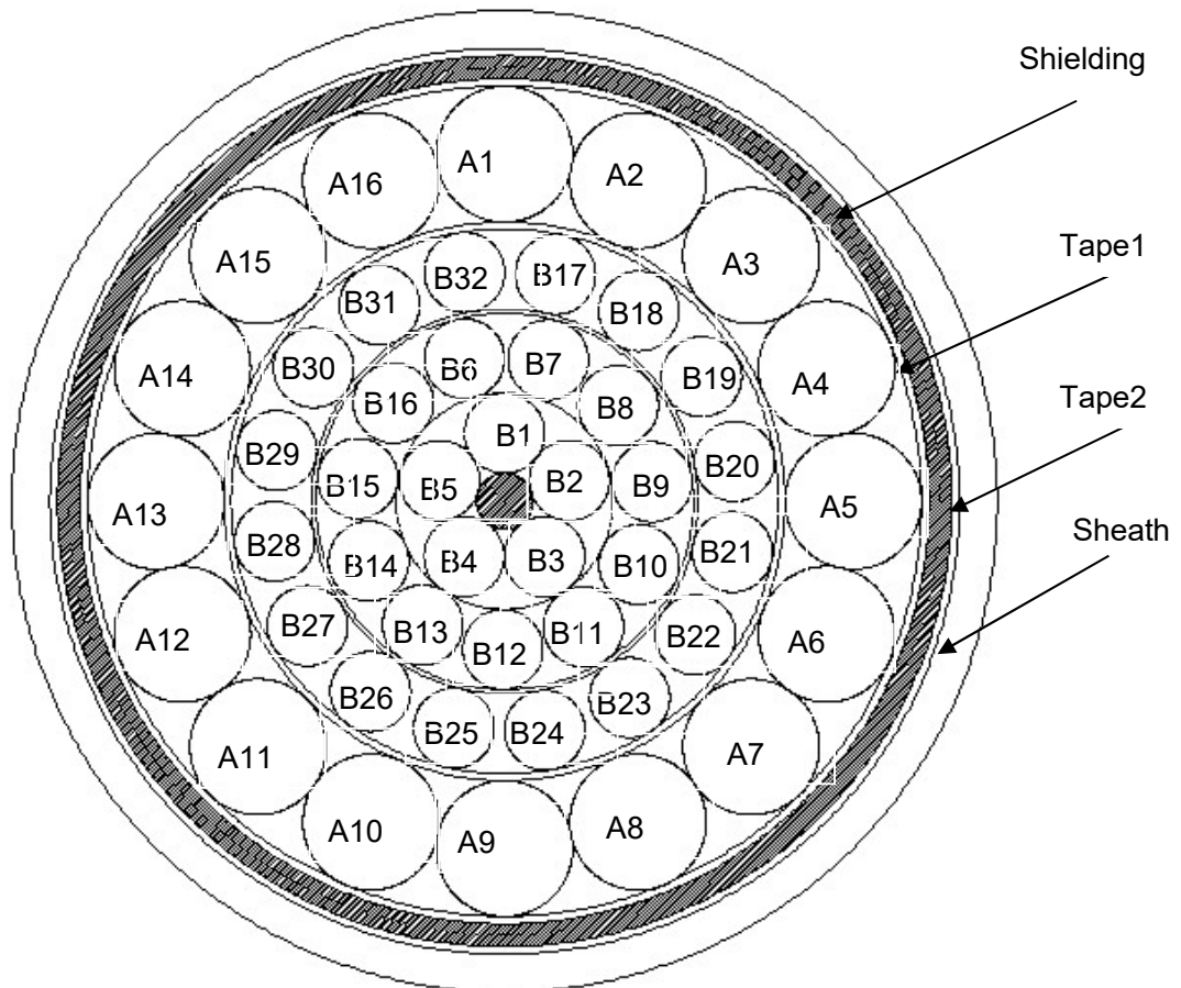
Fig.1 Cross section view of cable
