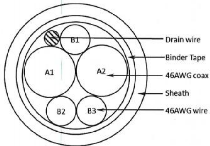
Fig.2 Cross-section view of cable
